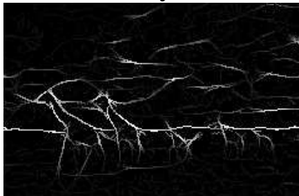
Boundary Prob.
