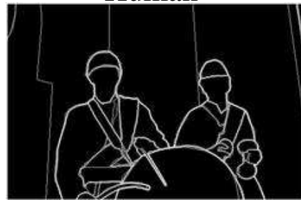
Canny
