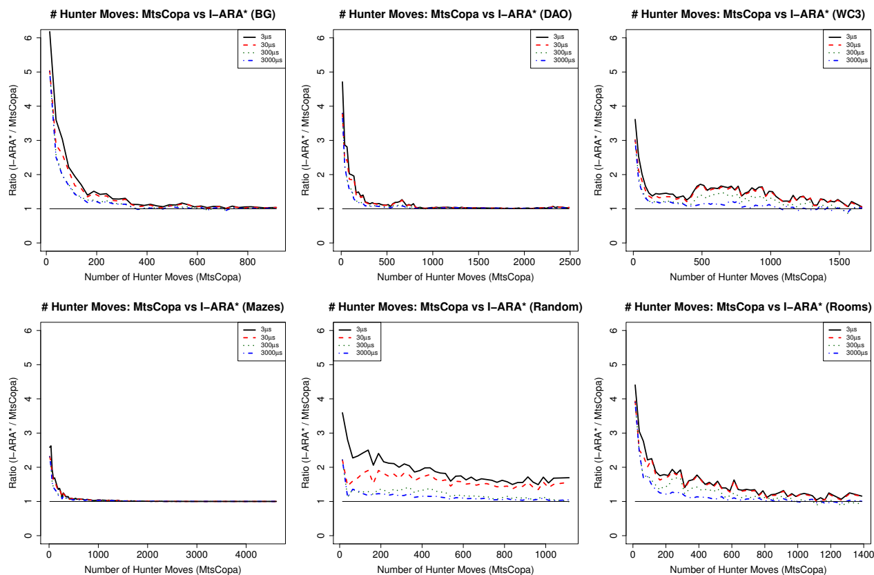
Figure 2: MtsCopa vs. I-ARA*. Relative improvement in the number of hunter moves taken by MtsCopa.
