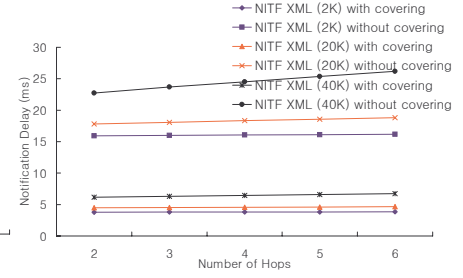
Figure 11. NITF XML
