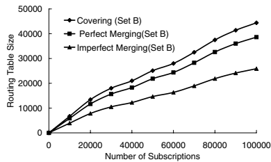
Figure 7. RTS
