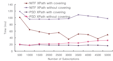
Figure 8. Process Time
