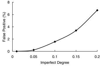
Figure 9. False Positives
