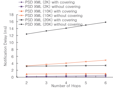
Figure 10. PSD XML
