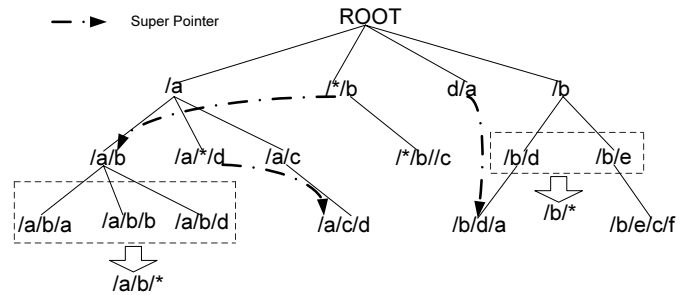
Figure 5. Subscription Tree
