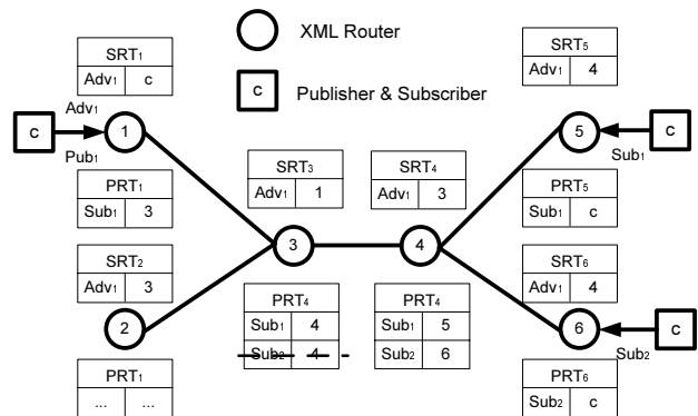
Figure 1. Content-based Routing
