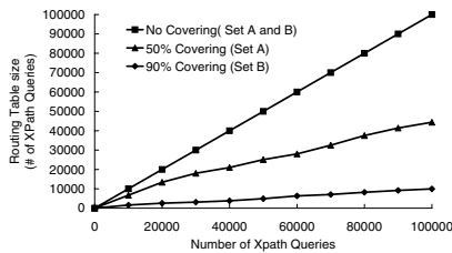
Figure 6. RTS
