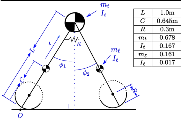
Fig. 2 The planar Anthropomorphic Walker and inertial parameters. The model parameters in the table are taken from Kuo (2002). Units of mass are given as a proportion of the total mass of the walker
