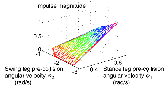
Fig. 4 Impulse magnitude \iota of the optimal cyclic gaits plotted versus pre-collision velocities \dot{\mathbf{q}}^- = (\dot{\phi}_1^-, \dot{\phi}_2^-) . During tracking, a bilinear fit to the data shown here is used to determine the conditional mean for a Gamma density over \iota at the beginning of each stride
