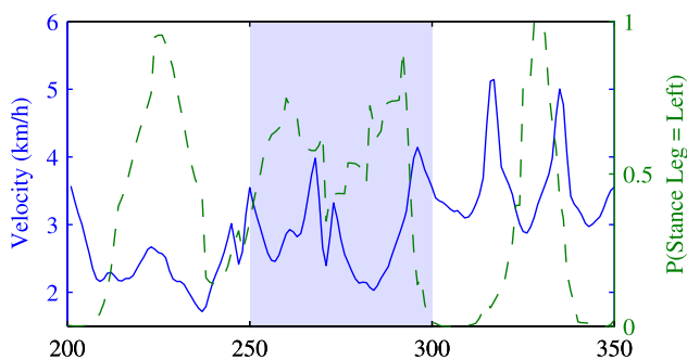
Fig. 13 (Color online) MAP trajectory velocity ( blue ) and stance leg posterior p(\text{stanceleg} = \text{left} | \mathbf{z}_{1:t}) ( dashed green ) for the times shown in Fig. 14. The highlighted region, corresponding to the middle row of Fig. 14, exhibits significant uncertainty about which leg is the stance leg
