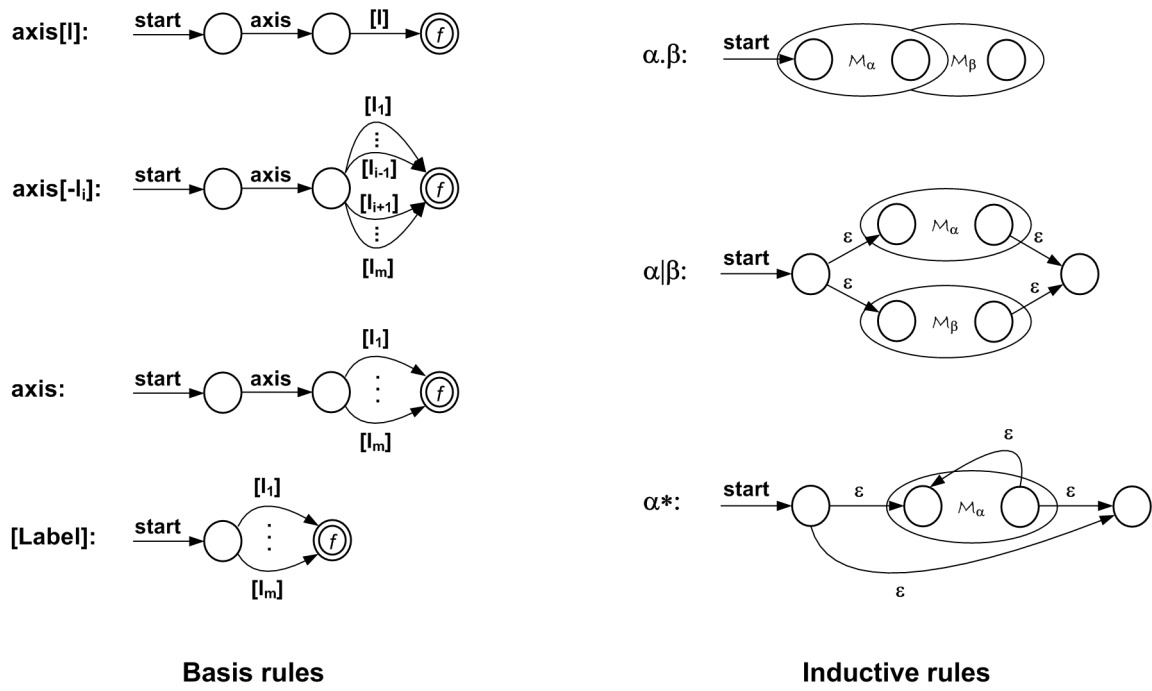
Figure 3.3: Rules of the modified Thompson's construction
