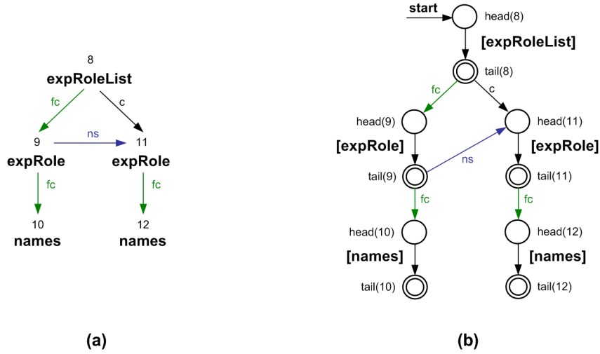
Figure 3.2: Axis graph fragment from node 8 (a) and its automaton \mathcal{M}_{\mathcal{A}}(8) (b)
