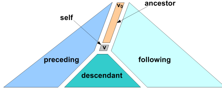
Figure 6.1: Partition of the nodes in the XML tree by axis relations
