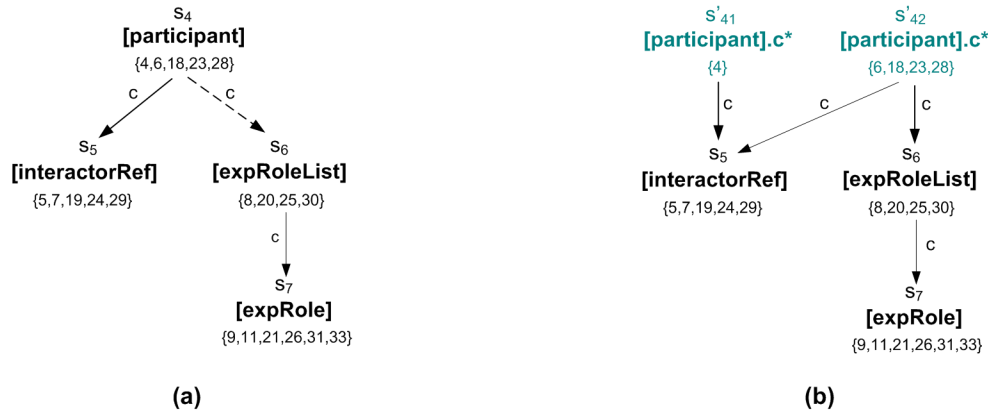
Figure 6.3: The [participant].c^* neighbourhood of s_4 from Figure 3.8: (a) before a c^* refinement, (b) after the refinement
