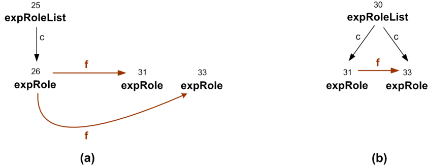
Figure 5.2: Two [expRoleList].c.f[expRole] neighbourhoods from our running example
