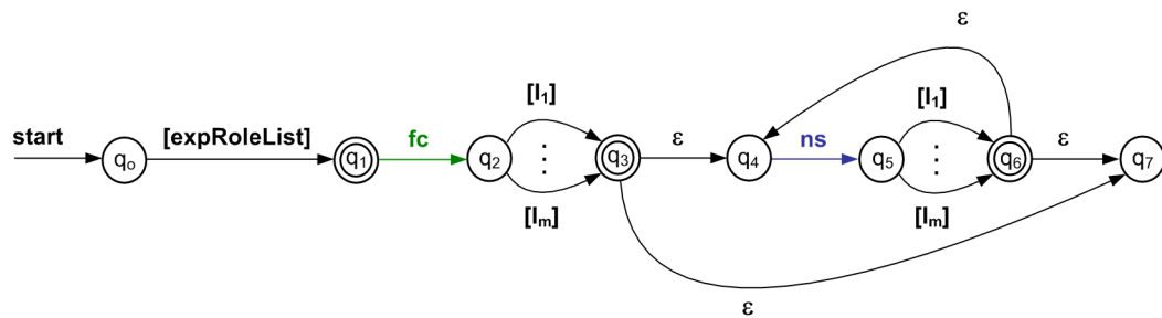
Figure 3.4: AxPRE automaton \mathcal{M}_{[expRoleList].fc.ns^*}
