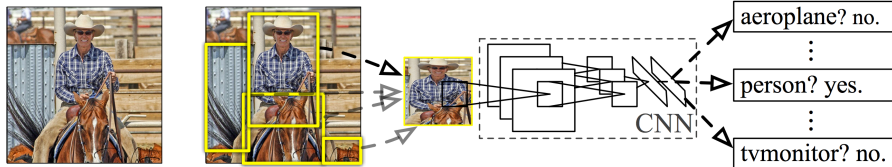
Figure: R. Girshick, J. Donahue, T. Darrell, J. Malik, Rich Feature Hierarchies for Accurate Object Detection and Semantic Segmentation, CVPR'14
