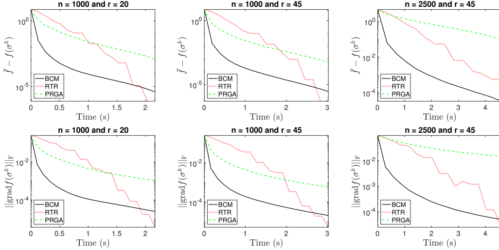
Figure 2: Convergence of the BCM algorithm versus RTR and PRGA algorithms, where the entries of A are drawn from a normal distribution.
