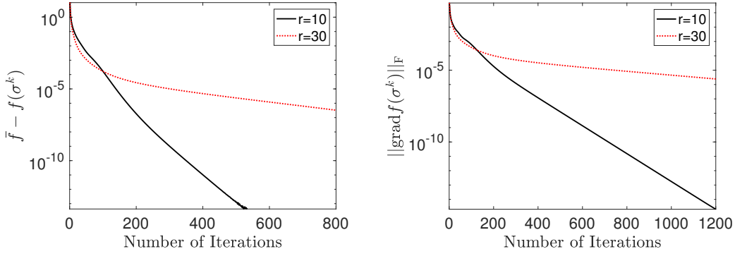
Figure 1: Convergence of the BCM algorithm, where the entries of A are drawn from a normal distribution and n = 500 . The local convergence can be observed to be linear.
