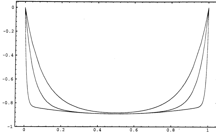
Test Problem 2: M(x) versus x
