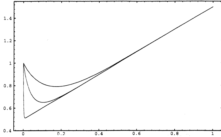
Test Problem 1: y(x) versus x
