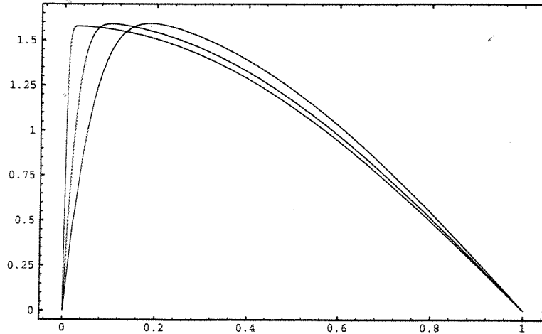
Test Problem 3: y'(x) versus x
