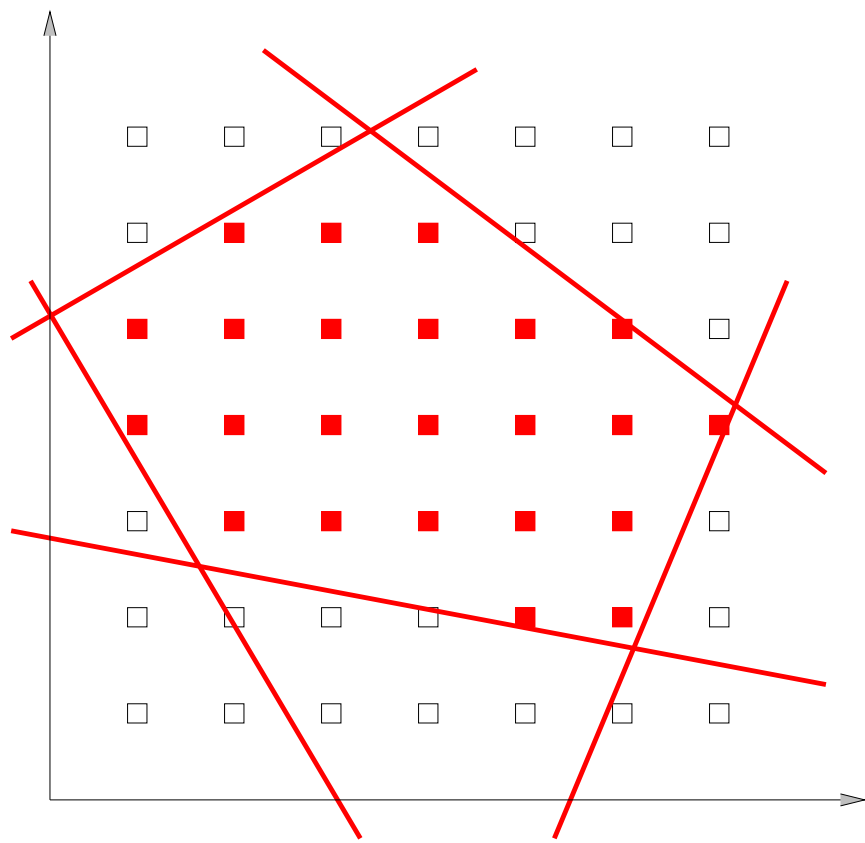
Figure 10 A Two-Dimensional Instance of MIP
