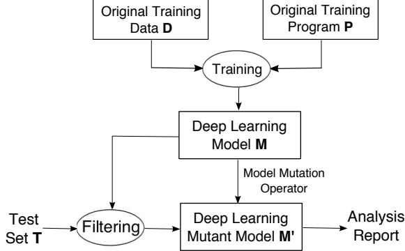
Fig. 5: The model level mutation testing workflow for DL systems.
