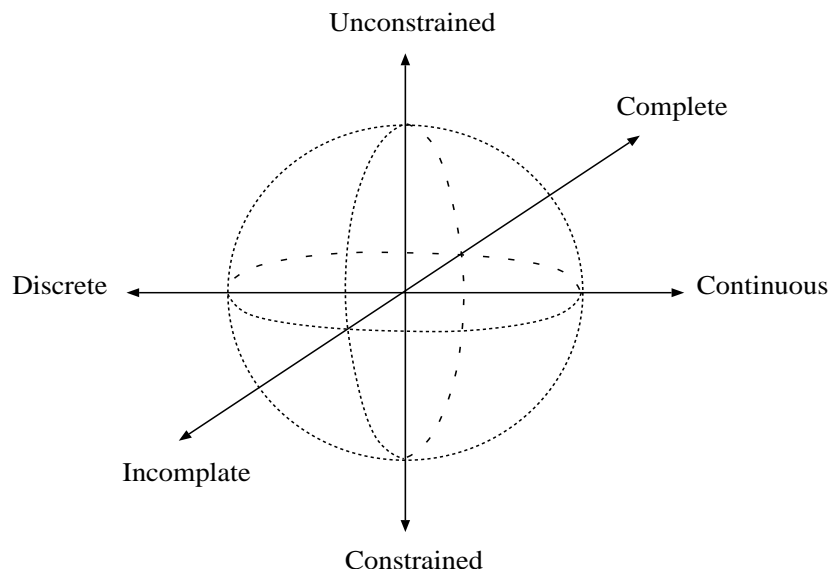
FIGURE 4. An algorithm space incorporating algorithm completeness for solving SAT. Each octant represents one class of SAT algorithms.
