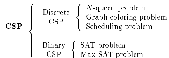
FIGURE 1. Some examples of the constraint satisfaction problem (CSP). SAT problem a special case of CSP, i.e., a CSP with binary values.
