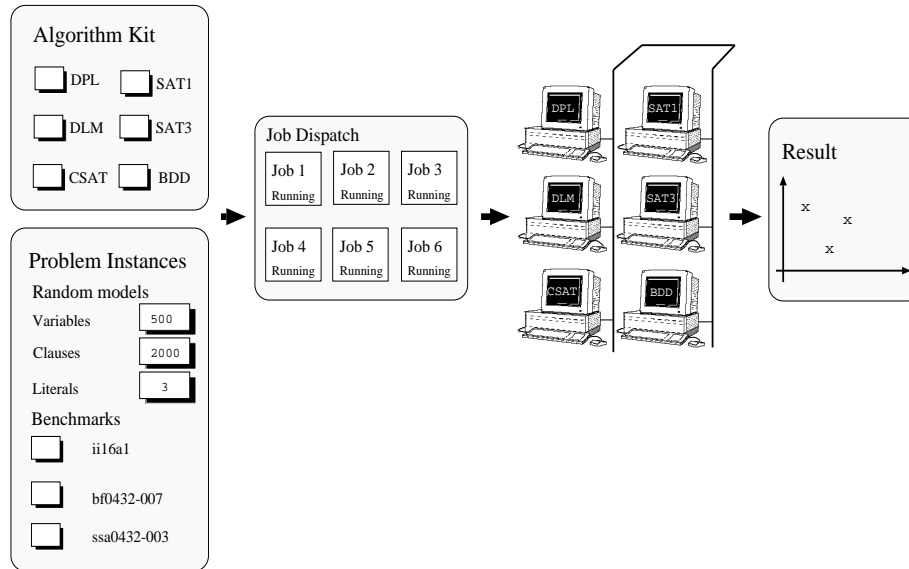
FIGURE 31. A software system, Cluster , for Multi-SAT algorithm.
