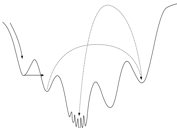
FIGURE 12. An informal example of the three-level search space model. A search process would go through an open search in the upper open portion of the search space, a peak search in the middle portion of the search space, and a trap search in the valley portion of the search space.
