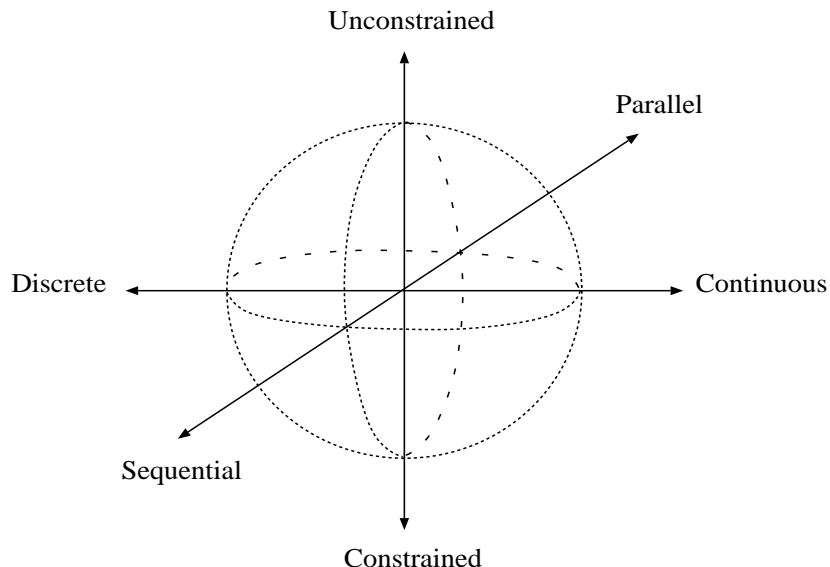
FIGURE 2. The algorithm space is a unified framework for discrete search algorithms and continuous optimization algorithms. The octants represent eight basic classes of algorithms.
