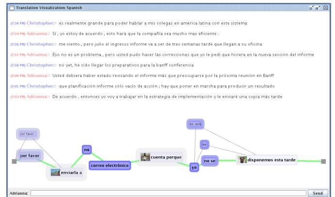
Figure 1: Translation uncertainty visualization in a chat interface: upper panel records chat history in the language of the user, lower panel displays the visualization of the most recently received message.
