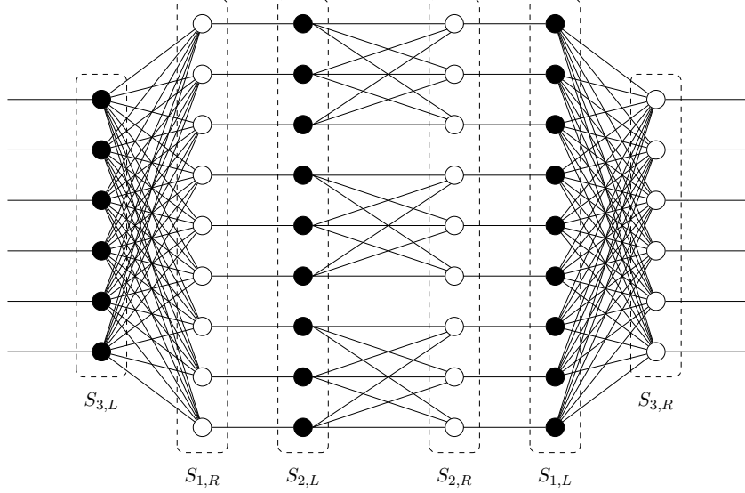
Figure 6: The Besser-Poloczek graph with parameter b = 3 . The edges on the left wrap around on the right connecting the nodes in S_{3,L} to the nodes in S_{3,R} .
