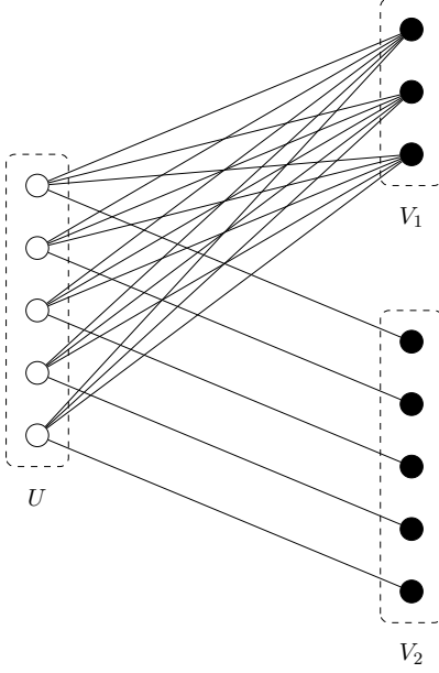
Figure 7: The H_{n,k} graph with n = 5 and k = 3 .
