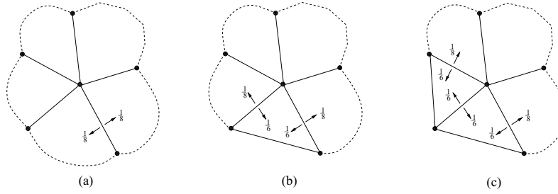
Fig. 3. Face contributions of edges for d(v) = 5 .
