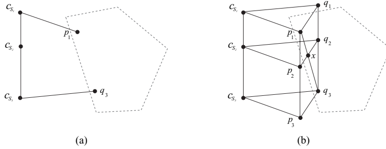
Fig. 6. The conflicting region is convex.
