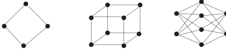
Fig. 1. Examples of inductive k -independent graphs for k = 2, 3, 4 .
