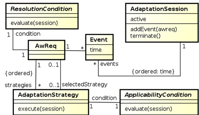
Fig. 6 Entities involved in the ECA-based adaptation process
