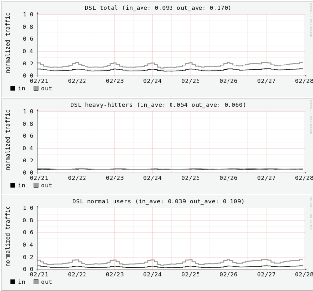
Figure 16: DSL weekly traffic: total DSL users (top), heavy-hitters (middle) and normal users (bottom)
