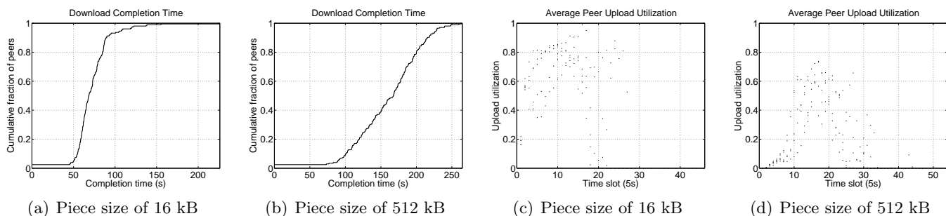
Figure 1: CDFs of peer download completion times and scatterplots of average upload utilization for five-second time intervals when distributing a 5 MB content (averages over 5 runs). Small pieces shorten download time and enable higher utilization.
