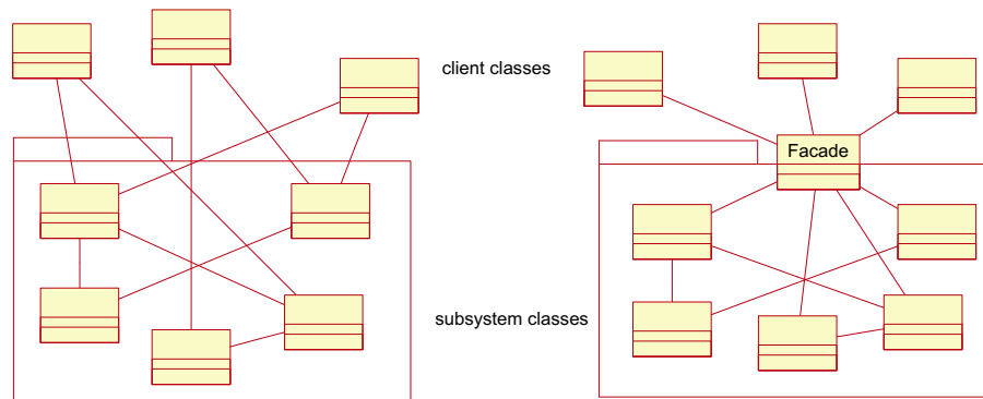
Fig. 5. The Facade design pattern (on the right)
