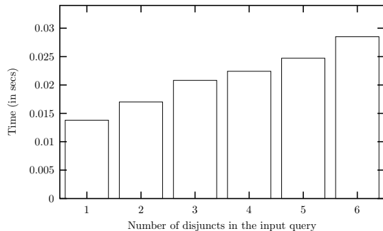
Figure 7: Translating large input queries
