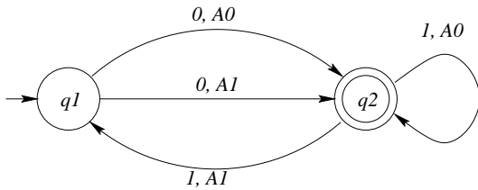
Figure 2: A graphical representation of a Büchi tree automaton accepting the tree from Figure 1.
