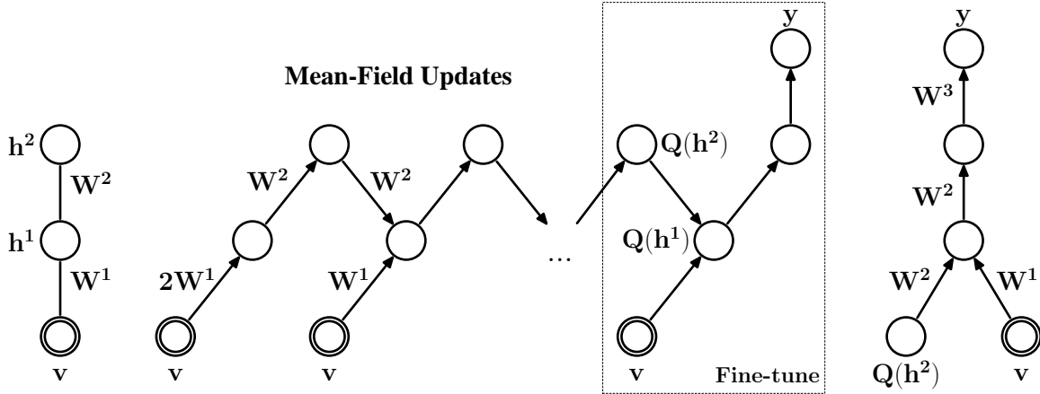
Figure 5.4: Left: A two-hidden-layer Boltzmann machine. Right: After learning, DBM is used to initialize a multilayer neural network. The marginals of approximate posterior q(h_j^2 = 1|\mathbf{v}) are used as additional inputs. The network is fine-tuned by backpropagation.
