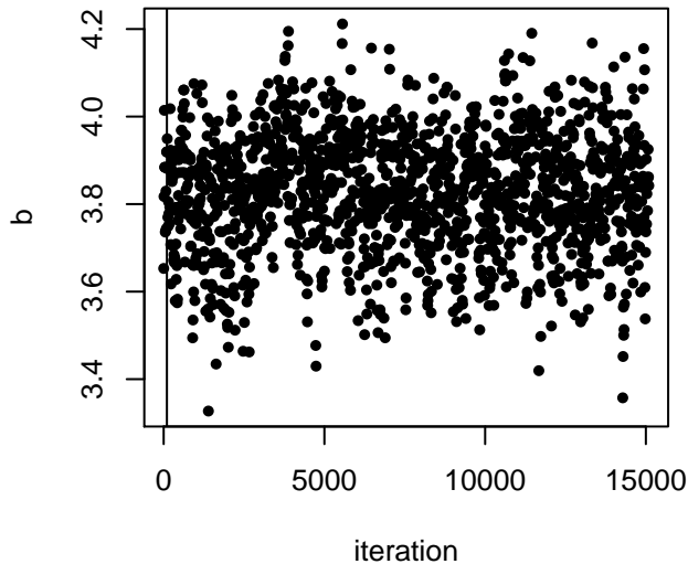
1st data set MCMC trace plot for b
