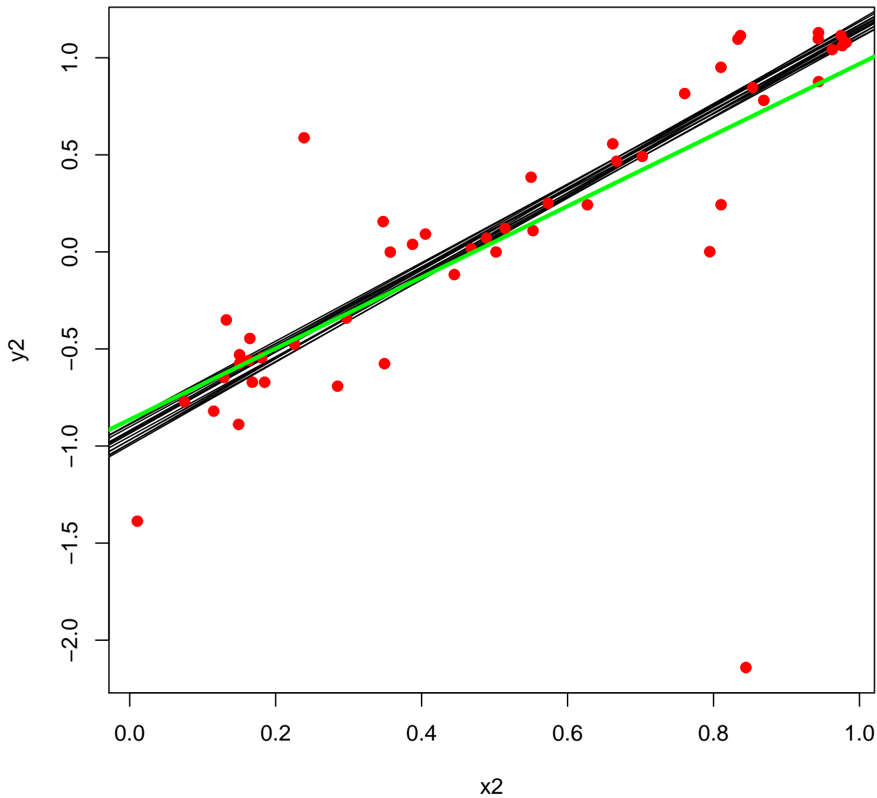
2nd data set fitted lines
