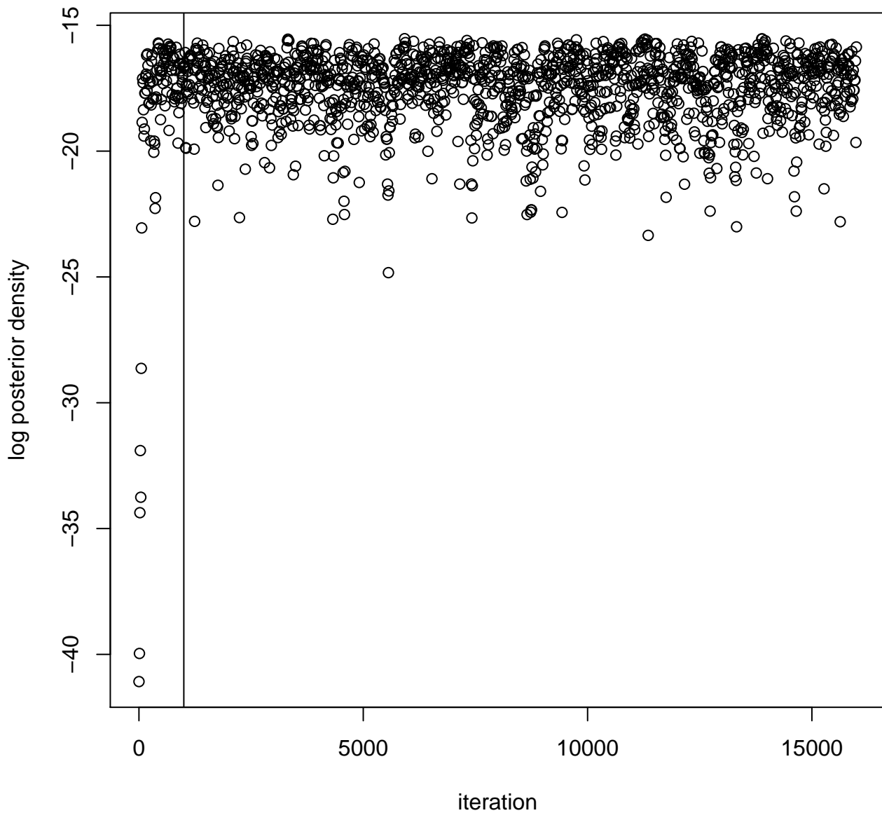
2nd data set trace plot of log posterior density
