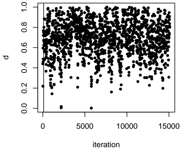
1st data set MCMC trace plot for d
