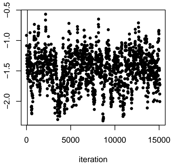
1st data set MCMC trace plot for s
