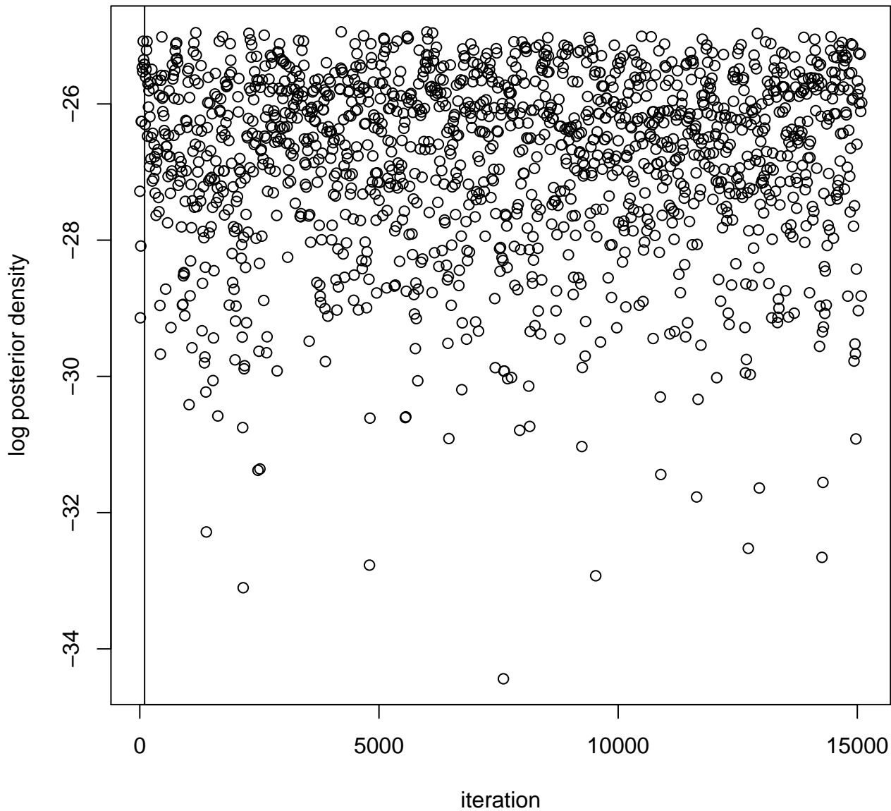
1st data set trace plot of log posterior density
