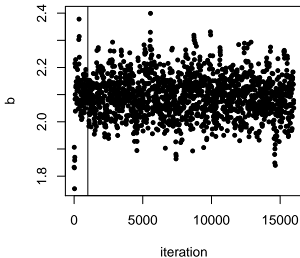
2nd data set MCMC trace plot for b
