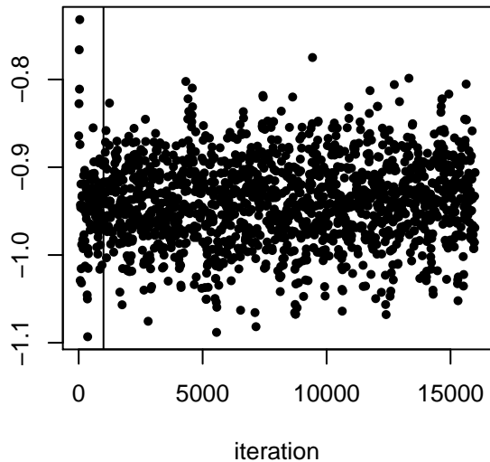
2nd data set MCMC trace plot for a
