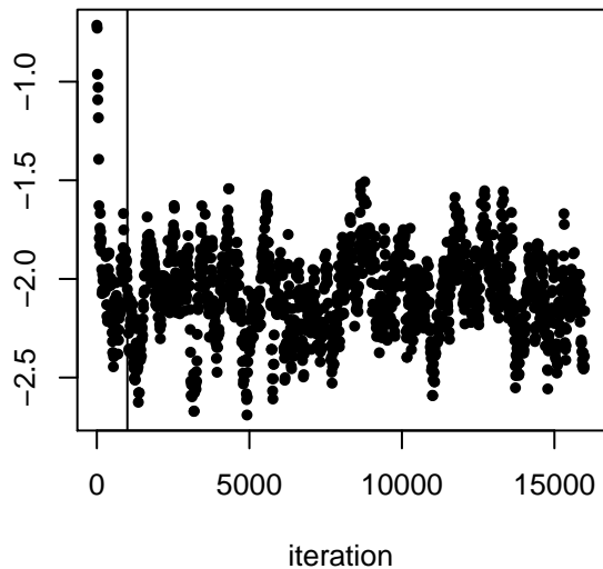
2nd data set MCMC trace plot for s
