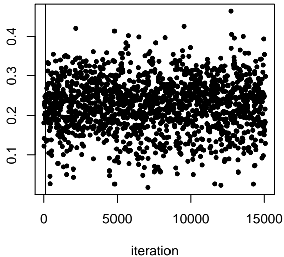
1st data set MCMC trace plot for a
