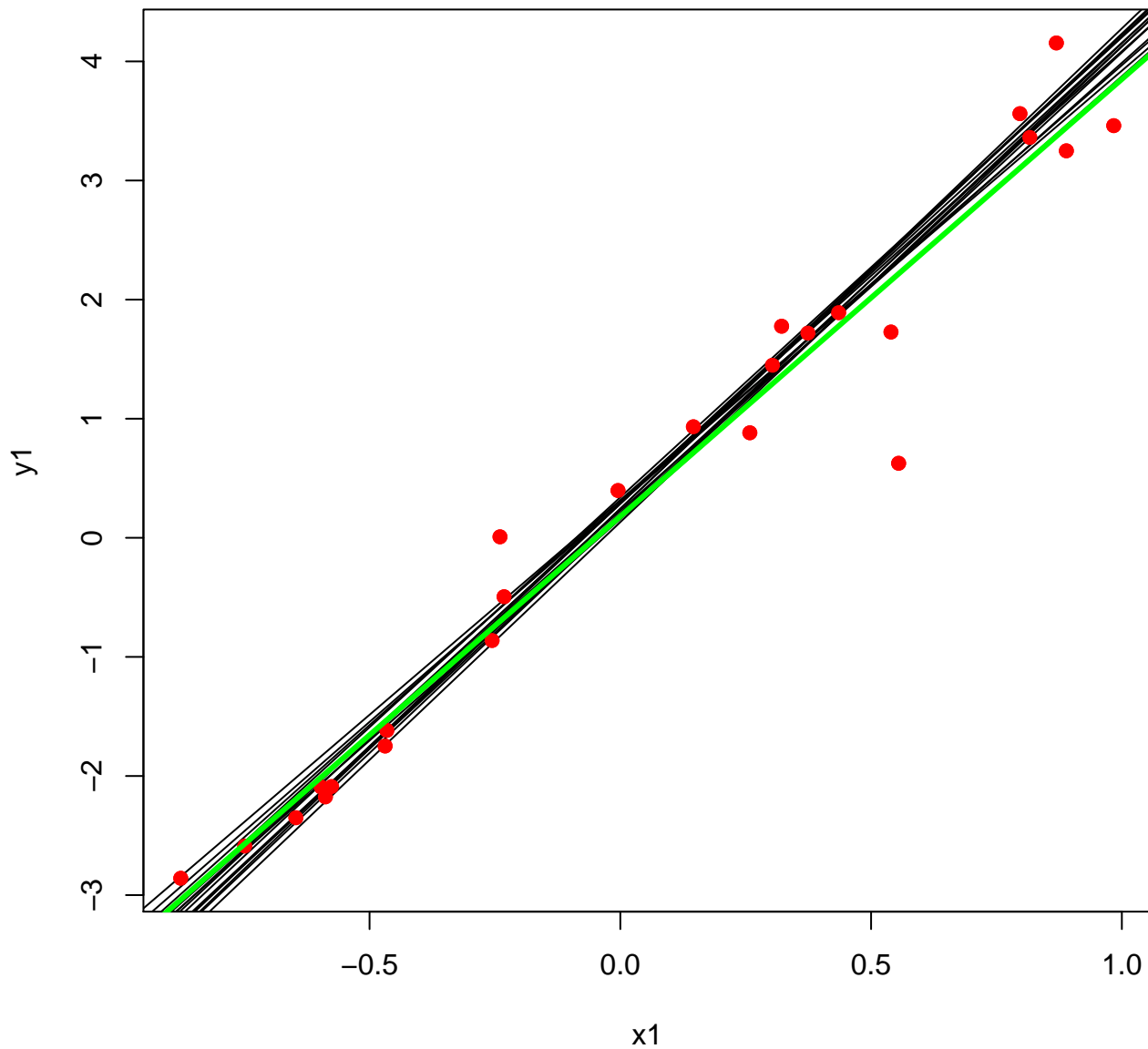
1st data set fitted lines
