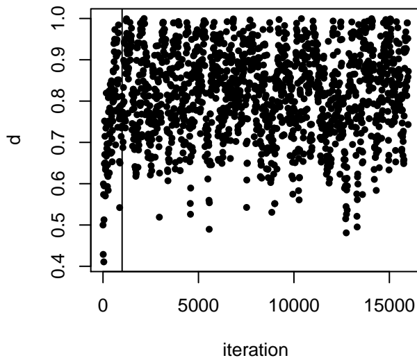
2nd data set MCMC trace plot for d
