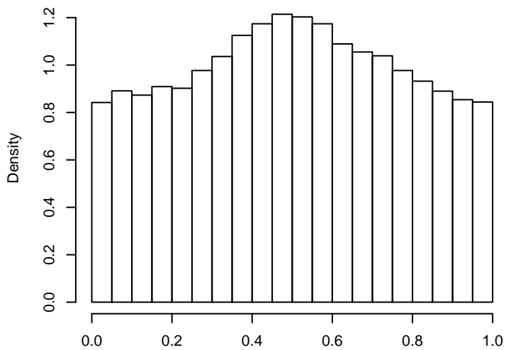
20000 pvalues for n = 2 and df = 3
