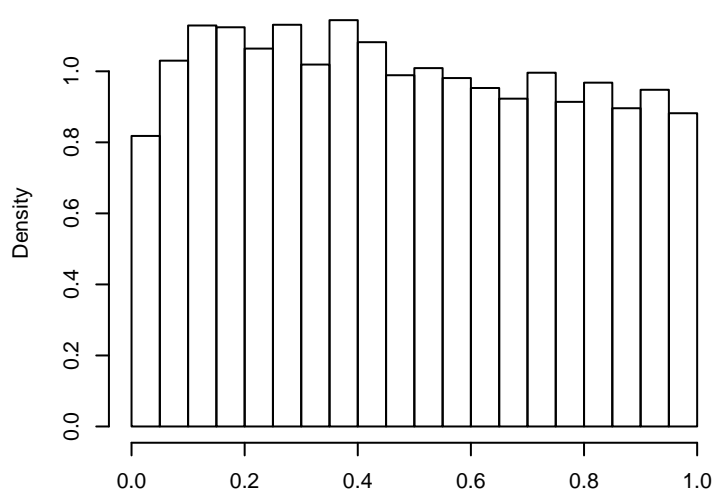
20000 pvalues for n = 20 and df = 3
