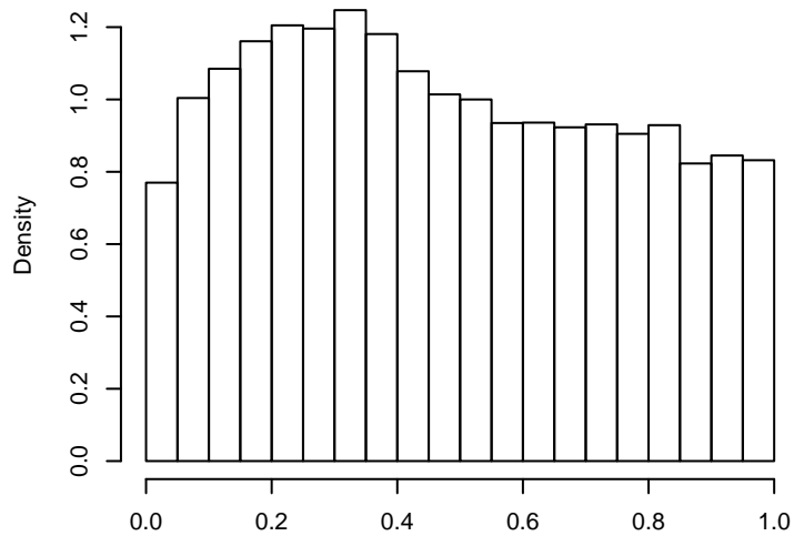
20000 pvalues for n = 20 and df = 2
