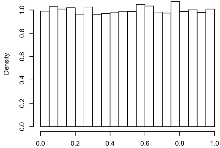
20000 pvalues for n = 20 and df = 100
