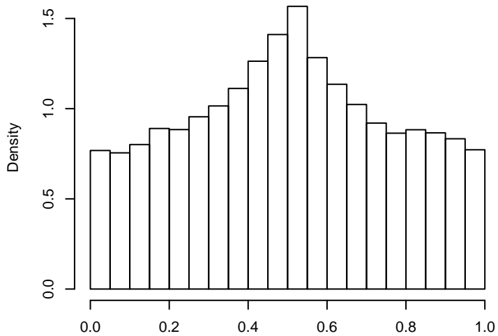
20000 pvalues for n = 2 and df = 2
