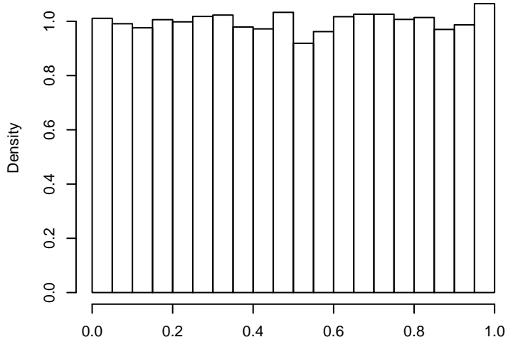
20000 pvalues for n = 2 and df = 100
