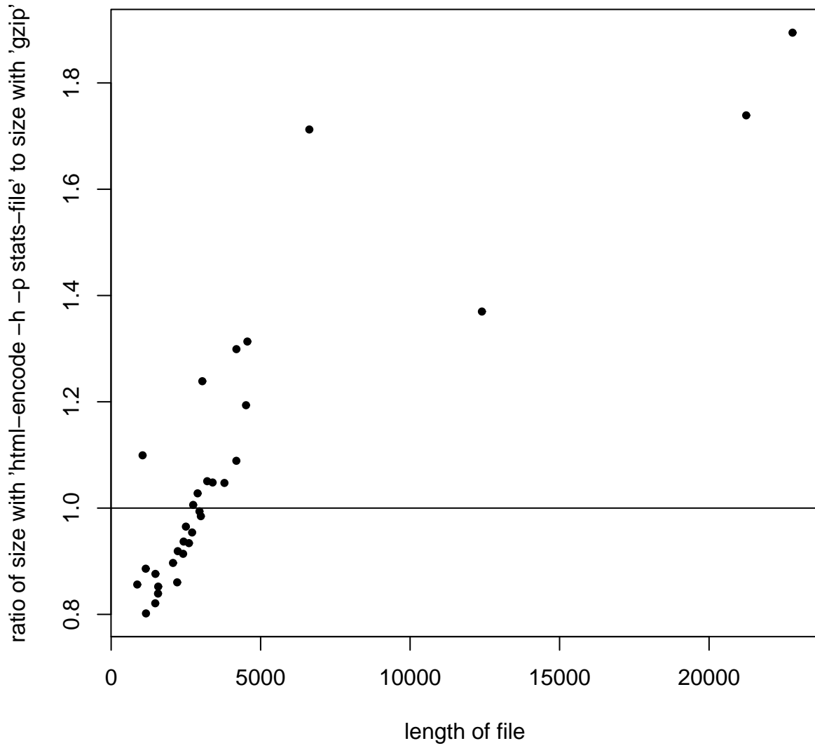
Comparison of compression performance on 32 test files
