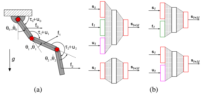
Figure 5: Three-link physical pendulum and network emulators. (a) An active pendulum with joint friction \tau_i , motor torques u_i , applied forces \mathbf{f}_i , and gravity \mathbf{g} . Without motor torques, the pendulum is passive. (b) Different types of emulators.
