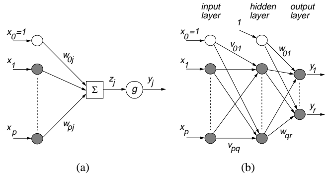
Figure 1: (a) Mathematical model of a neuron j . (b) Three-layer feedforward neural network N . Bias units are not shaded.
