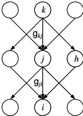
Figure 3: Units in a belief network.
