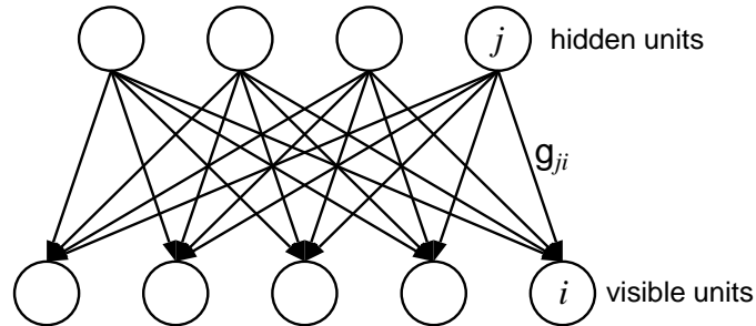
Figure 1: A generative neural network for mixtures of Gaussians.
