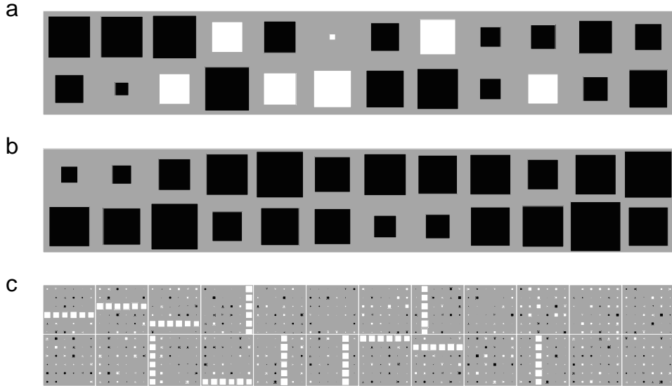
Figure 8: Generative weights of a three-layered RGBN after being trained on the noisy bars problem. a) Weights from the top layer hidden unit to the 24 middle-layer hidden units. b) Biases of the middle layer hidden units, and c) weights from the hidden units to the 6 \times 6 visible array, arranged in the same manner as in a).
