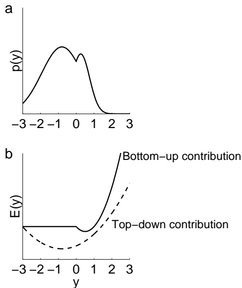
Figure 5: a) Schematic of the posterior density of an unrectified state of a unit. b) Bottom-up and top-down energy functions corresponding to a.
