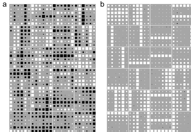
Figure 9: a) Generative weights of a factor analyzer with 24 hidden units trained on the same data as the RGBN. b) Generative weights of a mixture of 24 Gaussians trained on the same data.
