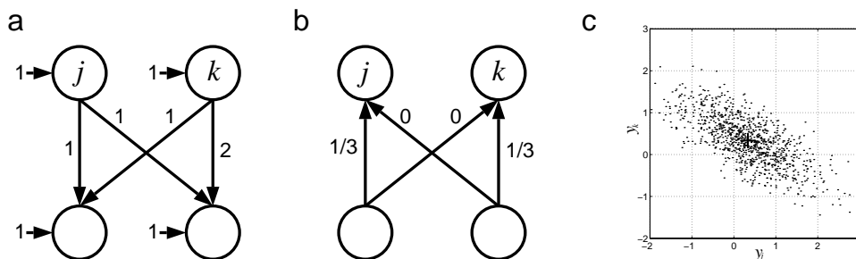
Figure 2: a) The hidden-to-visible generative weights and the hidden and visible local noise variances for a simple factor analysis model. b) The surprising visible-to-hidden recognition weights that compute the data-dependent mean of the posterior distribution in the two-dimensional hidden space. c) Samples from the posterior distribution in hidden space given the data point (1, 1) . The covariance of the posterior depends on the scalar product of the generative weight vectors of the two hidden units. In this example the positive scalar product leads to explaining away which shows up as a negative correlation of the two hidden variables.
