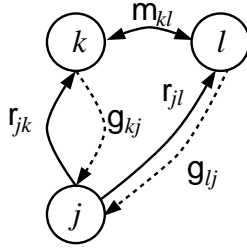
Figure 6: A network which, in addition to the generative connections, has bottom-up and lateral connections for performing perceptual inference.
