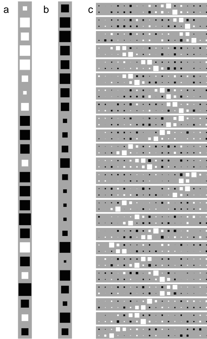
Figure 11: Generative weights of a three-layered RGBN after being trained on the stereo disparity problem. a) Weights from the top layer hidden unit to the 24 middle-layer hidden units. b) Biases of the middle layer hidden units, and c) weights from the hidden units to the 2 \times 18 visible array.
