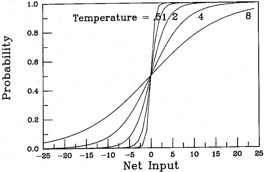
FIGURE 6. Probability of attaining value 1 as a function of the distance of the input of the unit from threshold. The function is plotted for several values of T .
