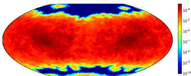
Figure 8: A Winkler-Tripel projection of the importance distribution of view directions, q^R , averaged over the thermus dataset at a typical iteration. Clearly visible is the equatorial belt of likely views, while axis aligned views (those on the top or bottom of the plot) are rarely seen.
