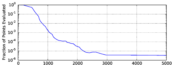
Figure 7: The fraction of quadrature points evaluated on average during optimization (horizontal axis is iterations). As resolution increases, the speedup obtained increases significantly yielding more than a 100,000 fold speedup.
