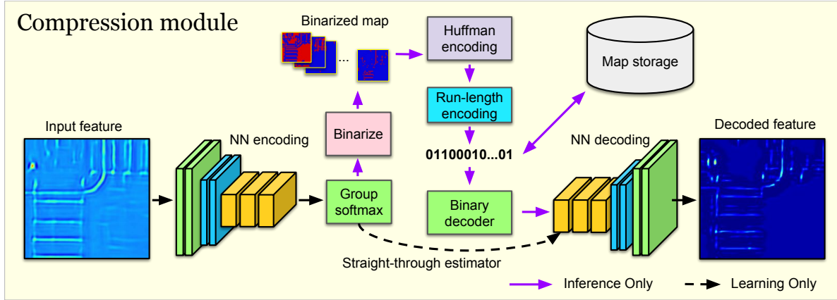
Figure 3: Our compression module. We obtain gradients for training with a straight-through estimator.
