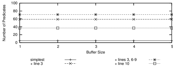
Figure 4: Plots for patched versions of testcases from the Apache example (Figure 2).
