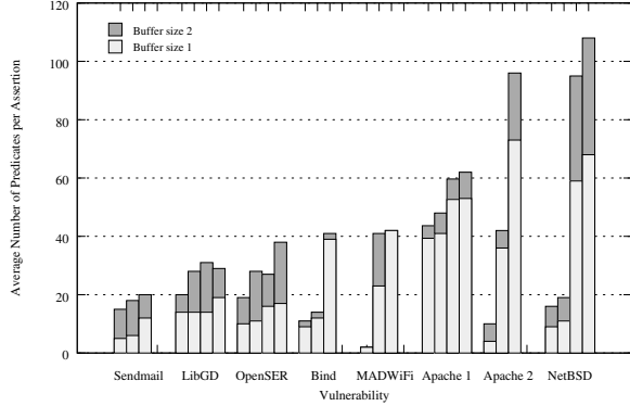
Figure 3: SatAbs performance variation over test-cases with vulnerabilities, buffer sizes 1 and 2.
