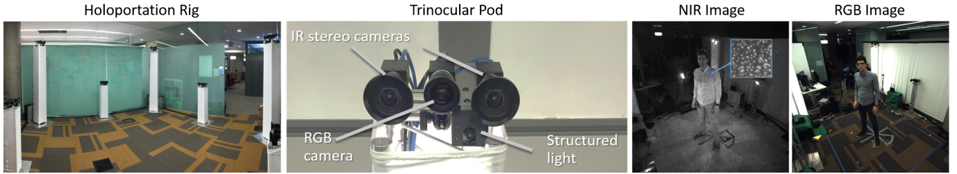
Figure 3. Left: Holoportation rig. Middle: Trinocular Pod. Right: NIR and RGB images acquired from a pod.
