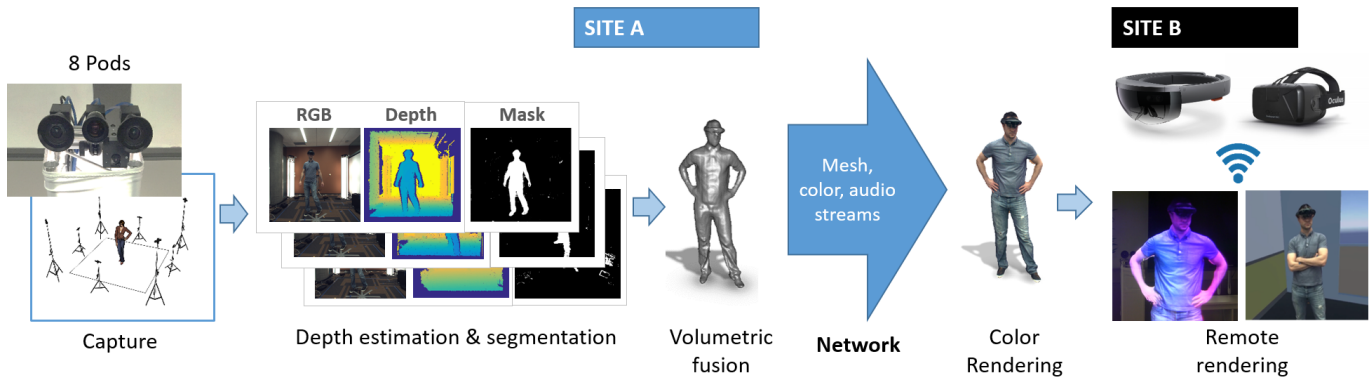
Figure 2. Overview of the Holoportation pipeline. Our capture units compute RGBD streams plus a segmentation mask. The data is then fused into a volume and transmitted to the other site. Dedicated rendering PCs perform the projective texturing and stream the live data to AR and VR displays.
