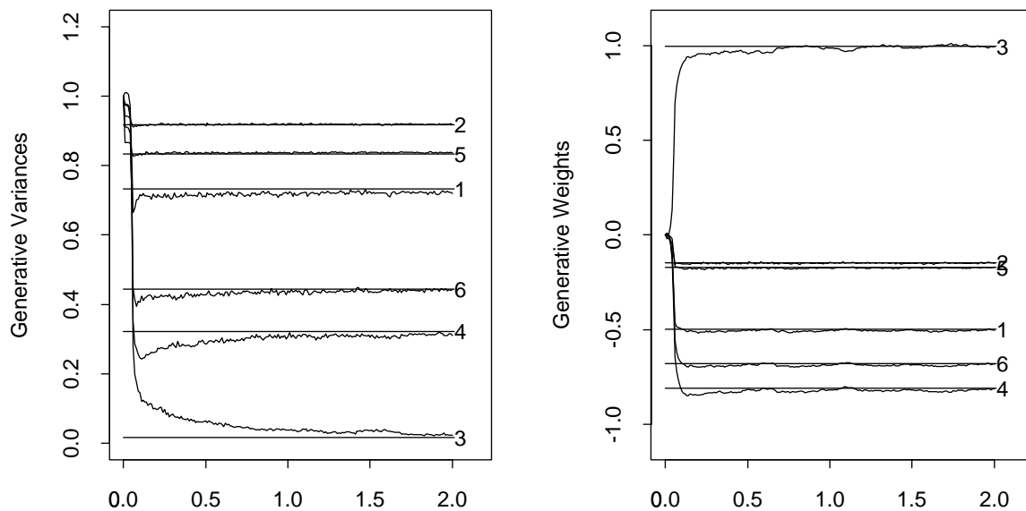
Figure 3: Wake-sleep learning of a single-factor model for six variables. The graphs show the progress of the generative variances and weights over the course of two million presentations of input vectors, drawn sequentially from a training set of size 500, with learning parameters of \eta = 0.0002 and \alpha = 0.999 being used for both the wake and the sleep phases. The training set was randomly generated from a single-factor model whose parameters were picked at random as described in Section 4.1. The maximum likelihood parameter estimates found by S-Plus are shown as horizontal lines.
