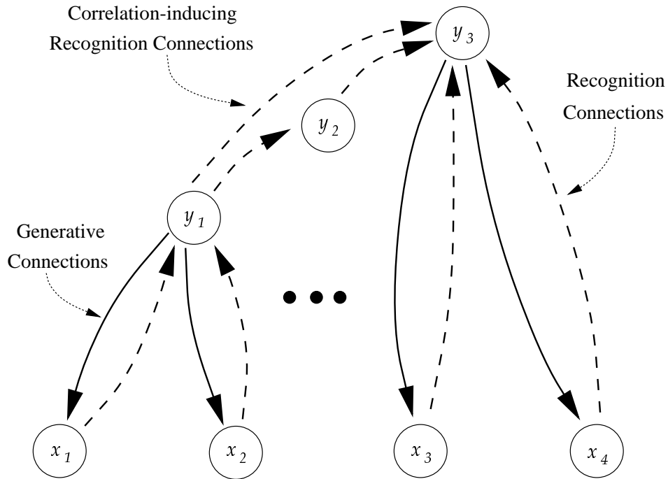
Figure 2: A Helmholtz machine implementing a model with three hidden factors, using a recognition model with a chain of correlation-inducing connections. The figure omits some of the generative connections from hidden factors to visible variables, and some of the recognition connections from visible variables to hidden factors (they are indicated by the ellipses). Note, however, that the only connections between hidden factors are those shown, which are part of the recognition model. There are no generative connections between hidden factors.
