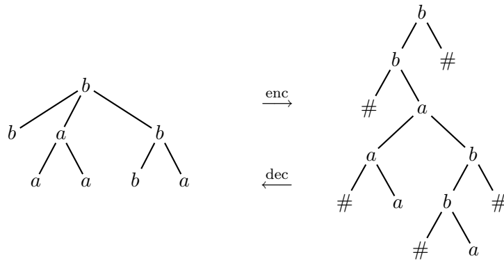
Figure 6: An unranked tree and its binary encoding.
