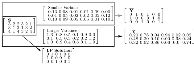
Figure 2. A “toy” example with a synthetic score matrix S , and matching results using LP (bottom) and the \bar{Y} approximation with two different variance matrices.
