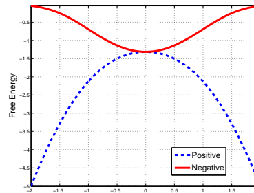
Figure 2: Free energy of a factored 3-way RBM with only one factor and one hidden unit as a function of the factor input, using a positive (dashed line) or negative (continuous line) factor-to-hidden matrix.
