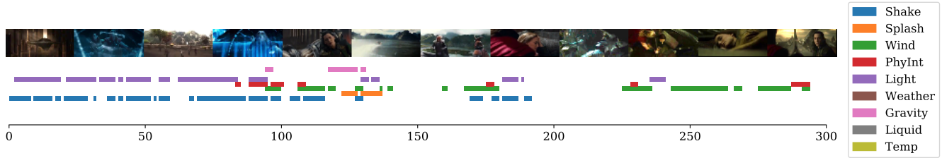
Figure 12: Example annotations made within a clip from the movie: Thor: The Dark World . We plot time on the x-axis and create a small rectangle for each effect type (based on color) corresponding to one second in the video. As can be seen, multiple effects do occur concurrently during intense scenes. On the other hand, possibly during dialog, effect annotations are sparse.
