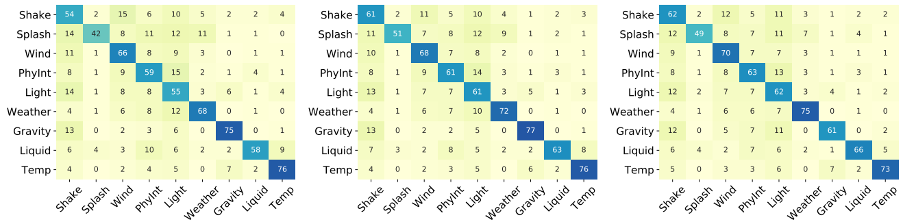
Figure 17: Effect correlation graph: we examine the causal effect of effects. For each sub-shot, we look ahead the next n subshots and see if the current effect has an impact on the next sub-shots. From left to right of the figure, n is 1, 5, 10 sub-shots ahead. We see that a strong diagonal for all plots indicating that effects of the same type tend to last for a long period of time, or occur again soon.
