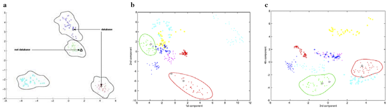
Fig. 30. Recognition of walking people from stereo data: walking motions from the training data are shown in the first four subspace dimensions. Each person is shown with a distinct color and symbol. Small black circles denote the estimated subspace coefficients, \alpha_i , obtained from video of people whose motions were included in the training set. The small black triangles depict subspace coefficients obtained from video of people whose motions were not included in the training set. (a) First two PCA components of a model learned from four subjects. Notice that in the first two dimensions the estimated coefficients for the test subject are easily confused with those of the training subjects. (b and c) First four components of a model learned with nine subjects. In the first four dimensions the motions of the training subjects cluster nicely, and the subspace coefficients estimated for a test subject do not lay close to any one cluster of the training subjects.
