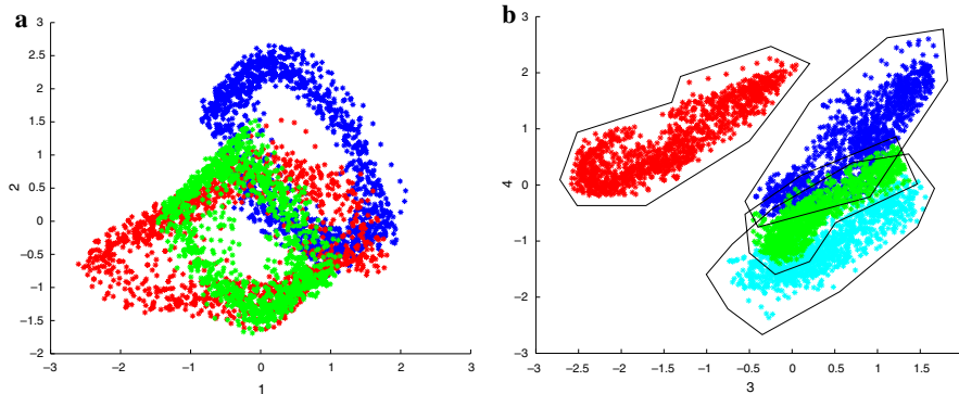
Fig. 5. Poor clustering in a pose subspace. The solid lines that delimited clusters have been manually done for visualization purposes. (a) Projection of training poses onto the first two eigen-directions of the pose subspace. (b) Projection of training poses onto the third and fourth eigen-directions of the pose subspace. While in the motion motion there is strong inter-subject separation, with the pose model in this figure, there is no inter-subject separation.
