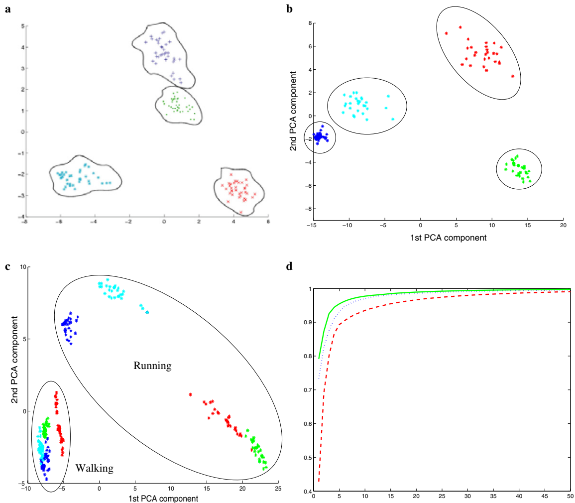
Fig. 1. Motion models. First two PCA components for (a) four different captures of four subjects walking at speeds varying from 3 to 7 km/h, (b) the same subjects at speeds ranging from 6 to 12 km/h, (c) the multi-activity database composed of the walking and running motions together. The data corresponding to different subjects is shown in different styles. The solid lines separating clusters have been drawn manually for visualization purposes. (d) Percentage of the database that can be generated with a given number of eigenvectors for the walking (dashed red), running (solid green) and the multi-activity databases (dotted blue). (For interpretation of the references to color in this figure legend, the reader is referred to the web version of this paper.)
