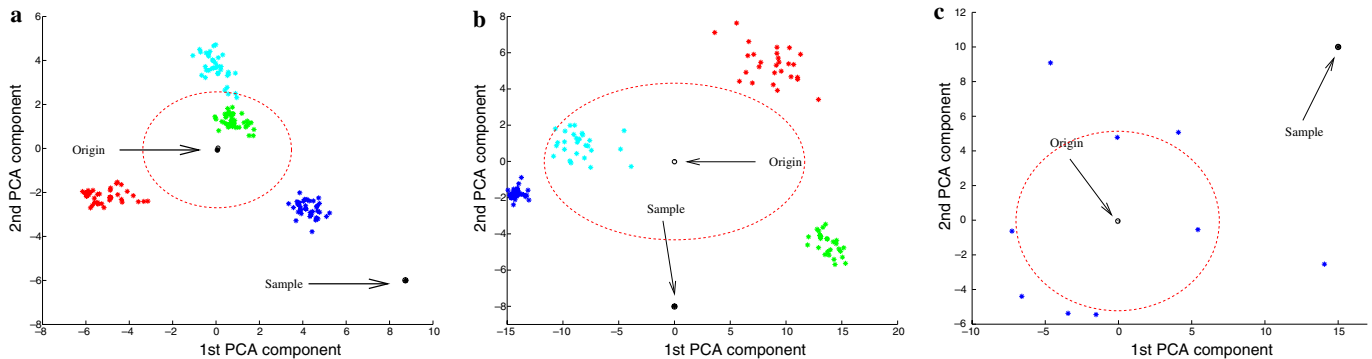
Fig. 6. Sampling the single activity databases. In each plot we show the most probable sample that is at the origin, and a sample with very low probability (far from the origin) for the (a) walking, (b) running, and (c) golfing databases. Their respective motions are shown in Fig. 7. The dashed curves are one standard deviation ellipses for the underlying Gaussian density model for the data.
