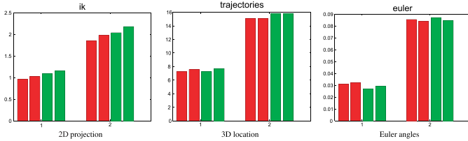
Fig. 20. Tracking mean errors as a function of the window size and the number of 2D constraints. Three types of errors (2D projection (pixels), 3D location (mm), Euler angles (radians)) are depicted. Each plot is split in two groups, the left one represents errors when tracking training data and the right one test data. For each group four error bars of two different colors are depicted, each color represents a different window size (3 on red, and 5 on green). For each color two bars show the errors first for the complete set of joints and then for the subset of joints, with similar results. Note that the estimated 3D joint location errors are very small, 0.7 cm in mean for the training data sequences, and 1.5 cm for the testing ones. (For interpretation of the references to color in this figure legend, the reader is referred to the web version of this paper.)
