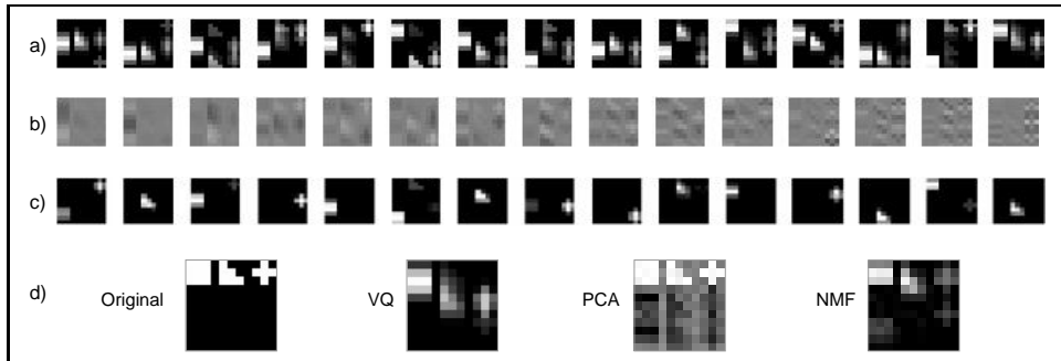
Figure 3: Other methods trained on shape images: a) VQ, b) PCA, and c) NMF. d) Reconstruction of a test image by the three methods (cf. Fig. 2c).
