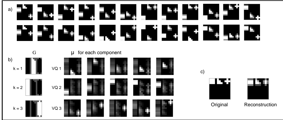
Figure 2: a) A sample of 24 training images from the Shapes dataset. b) A typical representation learned by MCVQ with 3 VQs and 5 states per VQ. c) Reconstruction of a test image: original (left) and reconstruction (right).
