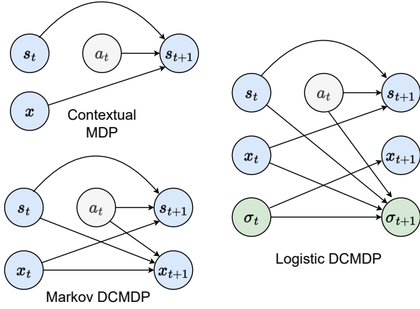
Figure 1: Causal diagrams comparing Contextual MDPs (Hallak et al., 2015), Markov DCMDPs (Section 2.1) and Logistic DCMDPs (Section 3). Logistic DCMDPs are history dependent, where \sigma_t = \sum_{l=0}^{t-1} \alpha^{t-l-1} \mathbf{f}_l^*(s_l, a_l, x_l) , and \mathbf{f}_l^* : \mathcal{S} \times \mathcal{A} \times \mathcal{X} \mapsto \mathbb{R}^M are unknown , non-stationary, vector valued feature mappings.
