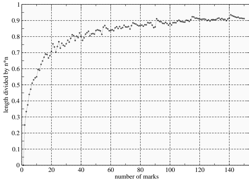
Figure 2.4: Smallest known values for G(n) divided by n^2
